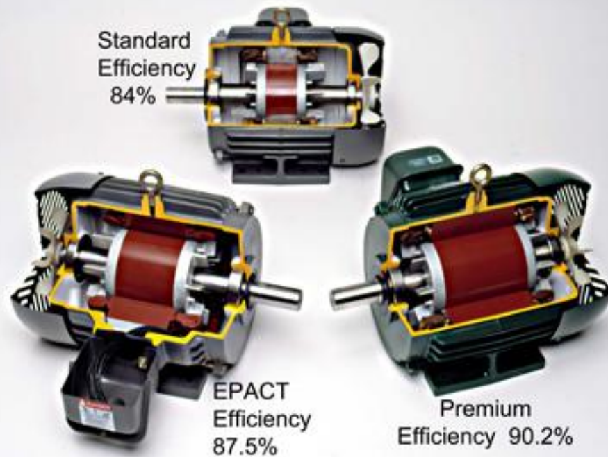
Figure 2: Motor Construction Each Motor is 10 HP, 1200 RPM
